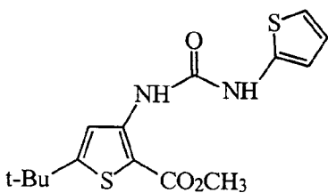
5-tert-Butyl-3-(3-thiophen-2-yl-ureido)-thiophene-2-carboxylic acid methyl ester
